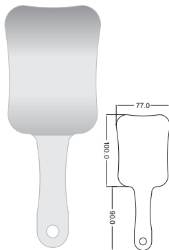
Occlusal-Large SSM-104
