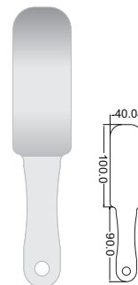
Lateral SSM-404
